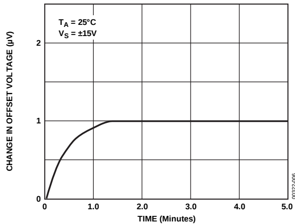
Figure 6. Warm-Up Drift
