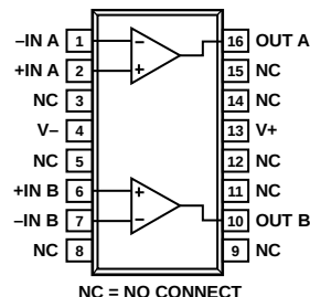
Figure 1. 16-Lead SOIC (S-Suffix)
