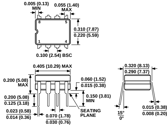
Figure 36. 8-Lead Ceramic Dual In-Line Package [CERDIP] (Q-8) Z-Suffix
