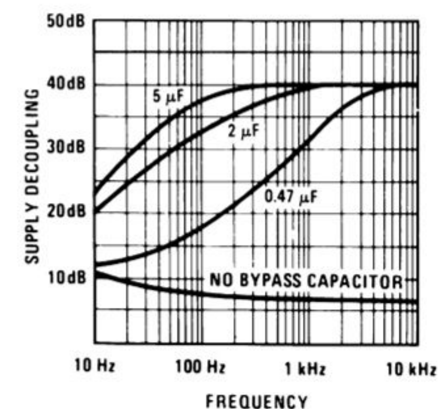
Supply Decoupling vs Frequency
