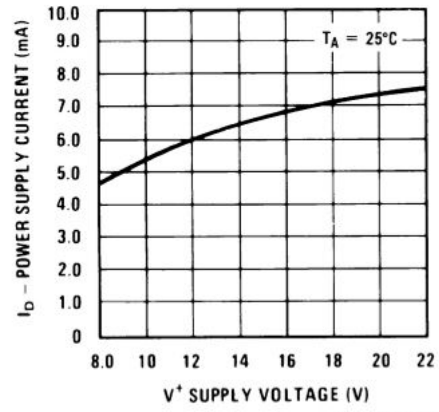
Power Supply Current vs Supply Voltage
