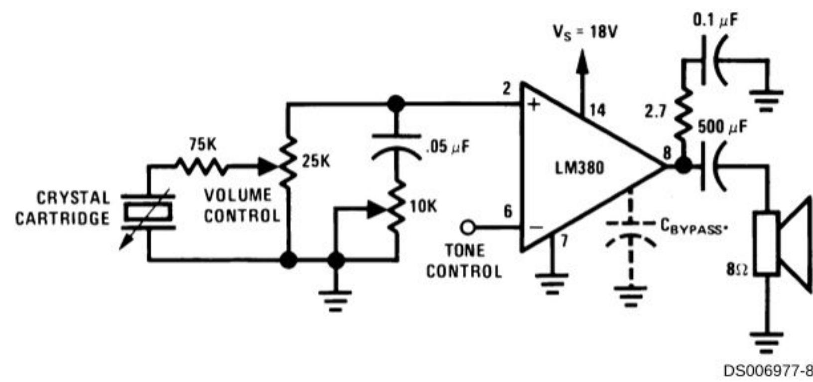
Phono Amplifier
