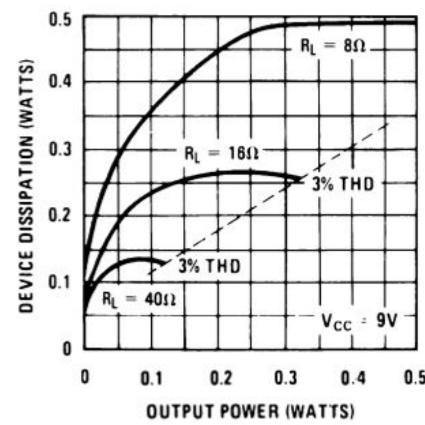
Device Dissipation vs Output Power
