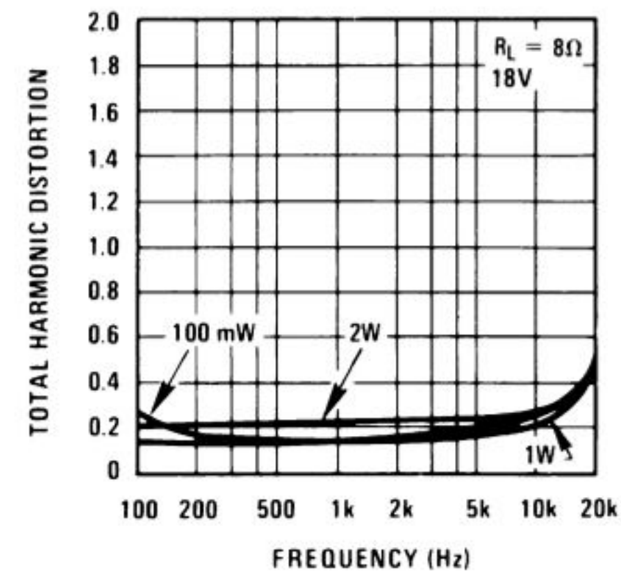
Total Harmonic Distortion vs Frequency
