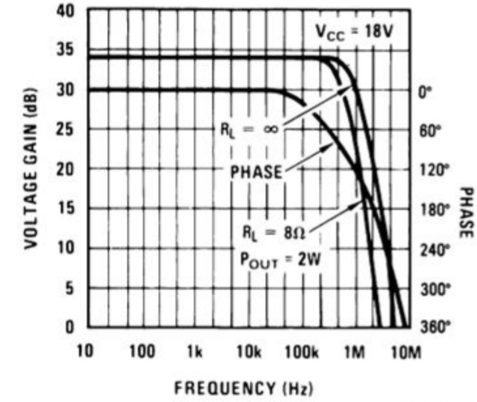
Output Voltage Gain and Phase vs Frequency
