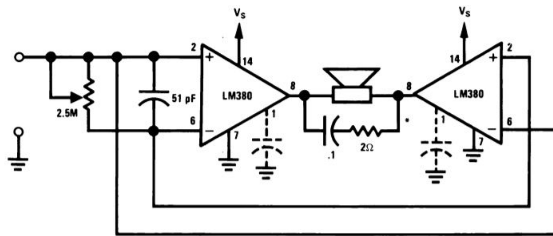
Bridge Amplifier
