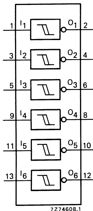
Fig.1 Functional diagram.
