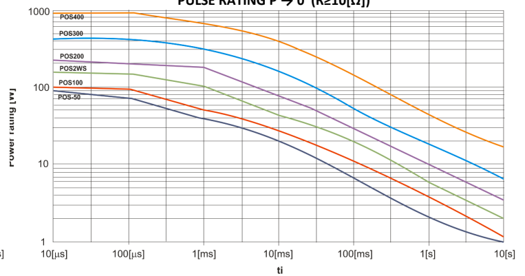
PULSE RATING P \rightarrow 0 ( R \geq 10[\Omega] )
