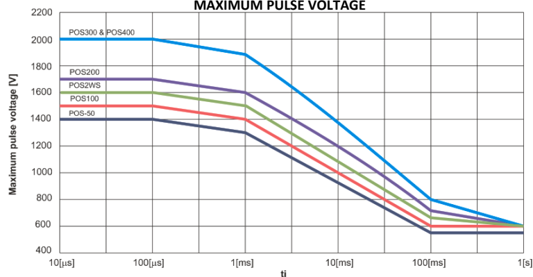
MAXIMUM PULSE VOLTAGE
