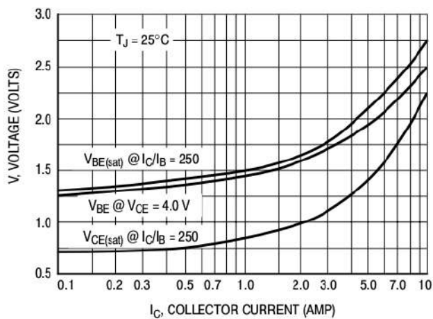
Figure 11. "On" Voltages
