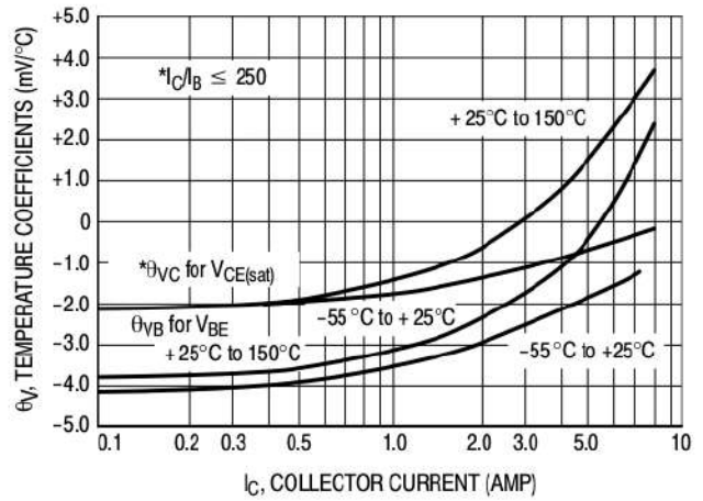
Figure 12. Temperature Coefficients
