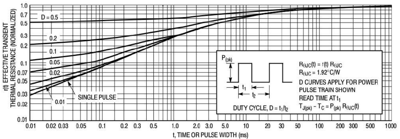
Figure 4. Thermal Response
