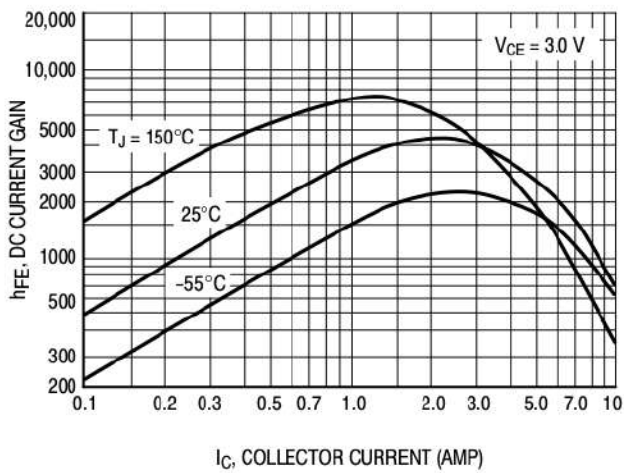
Figure 9. DC Current Gain
