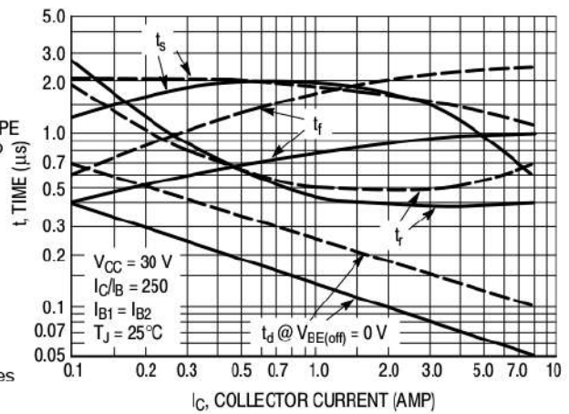
Figure 3. Switching Times
