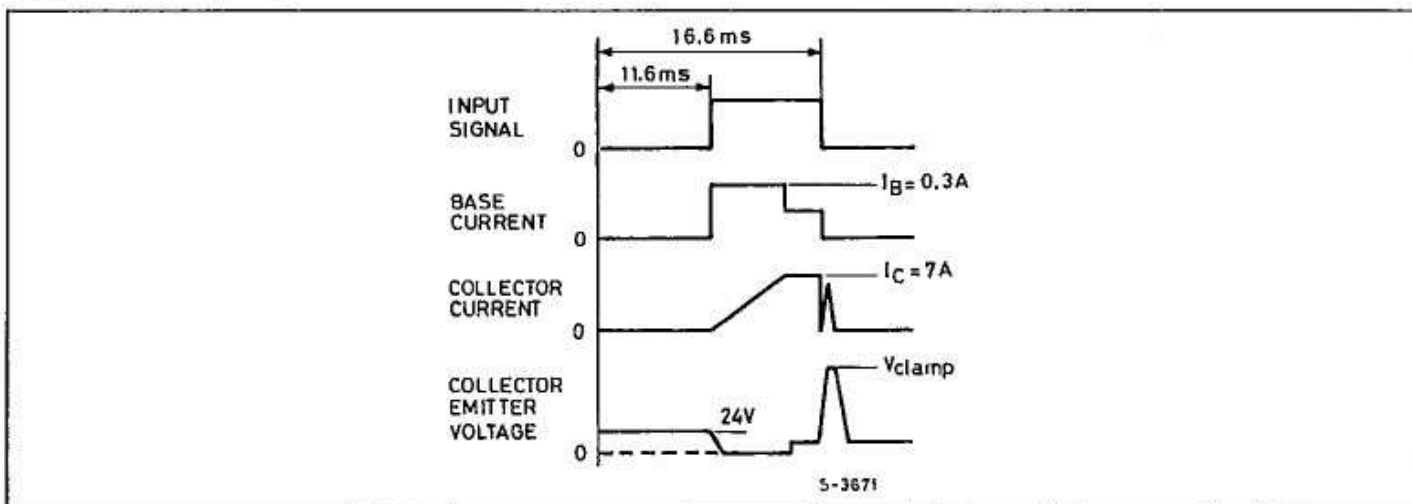
Figure 3 : Functional Test Waveforms.
