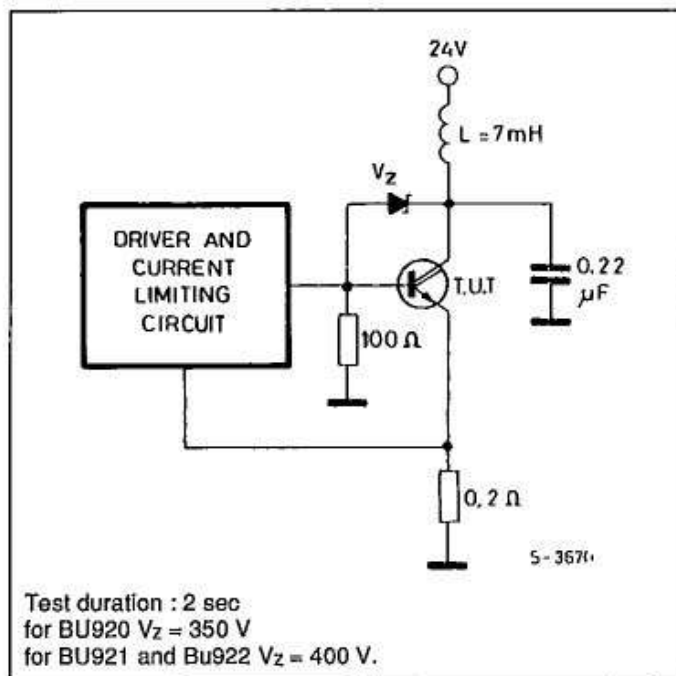
Figure 2 : Functional Test Circuit.
