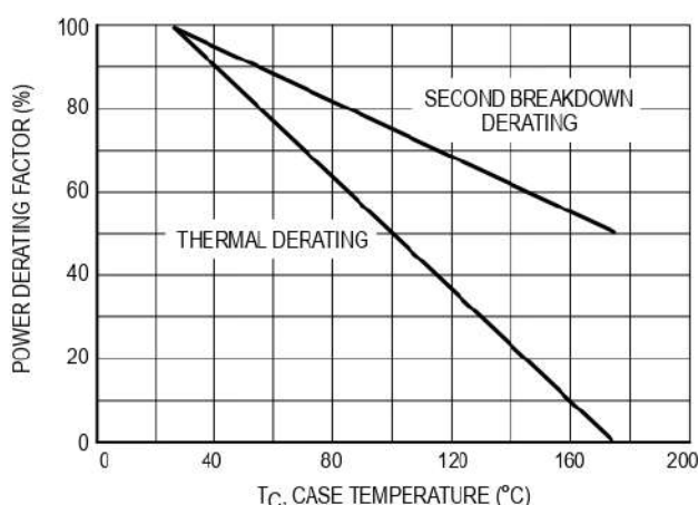
Figure 14. Power Derating
