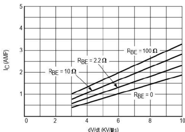
Figure 17. I_C = f(dV/dt)
