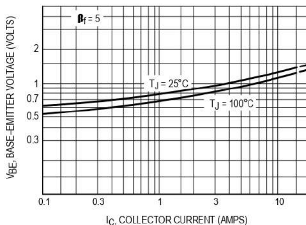
Figure 4. Base-Emitter Voltage
