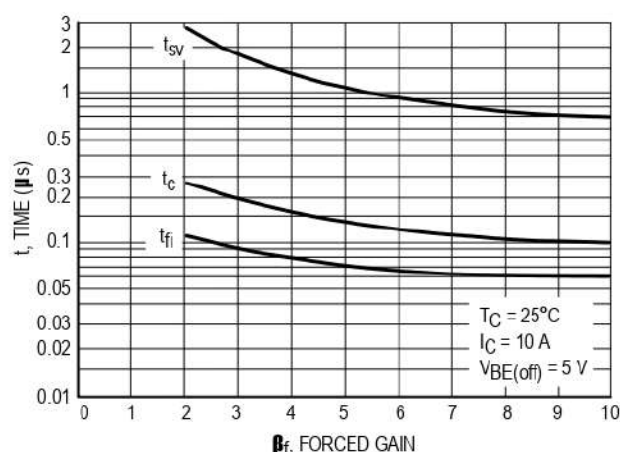
Figure 11a. Turn-Off Times versus Forced Gain
