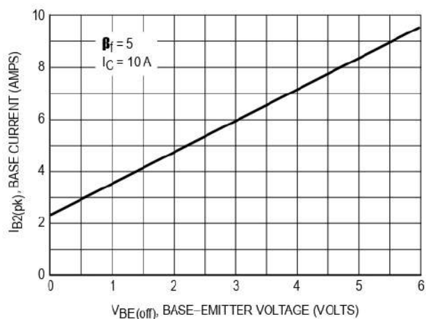
Figure 8. Peak–Reverse Current
