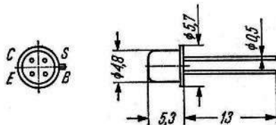
Rys. 1-450. BF173
