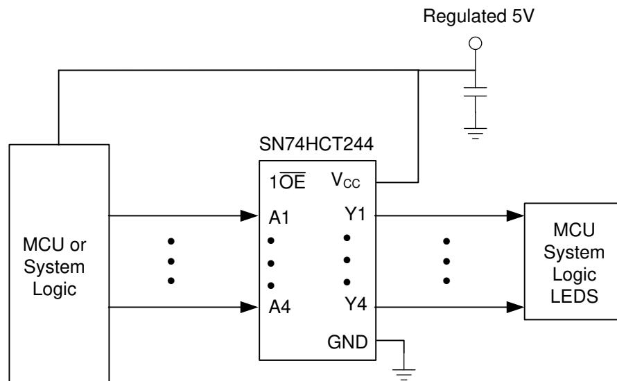
Figure 8-1. Application Schematic
