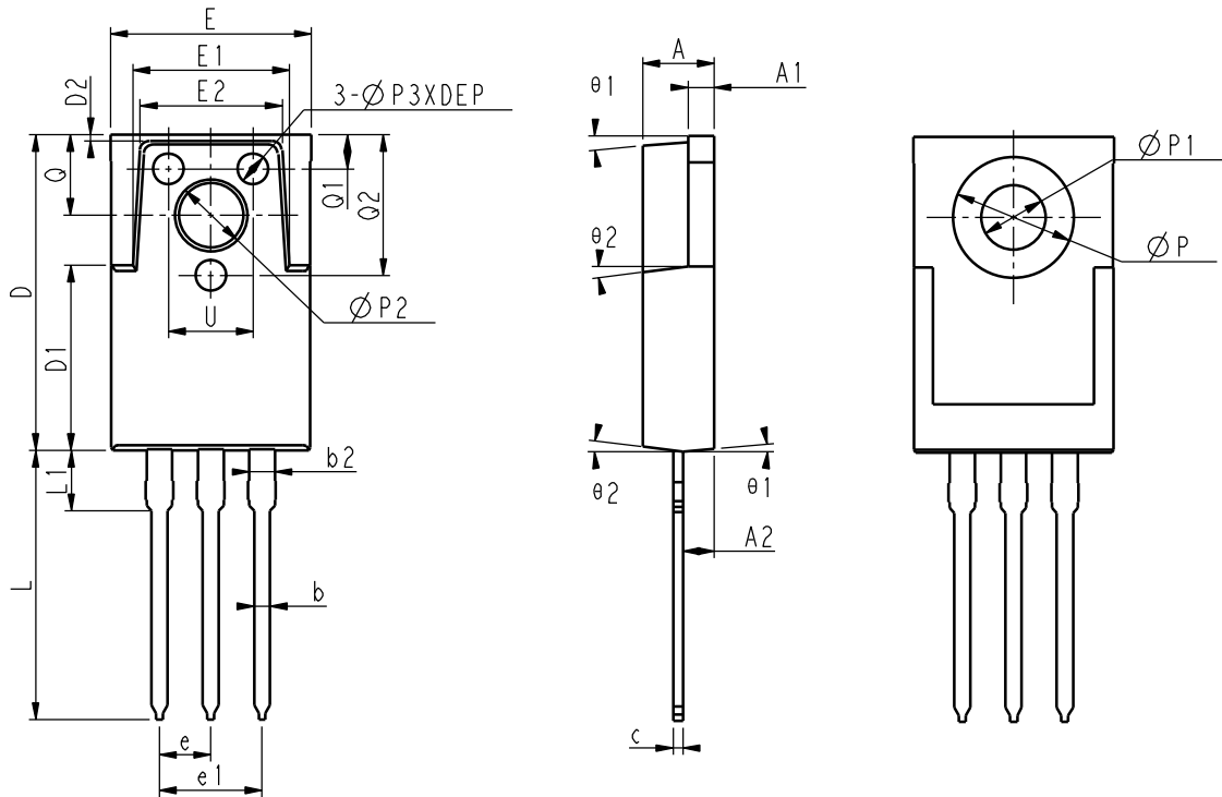
COMMON DIMENSIONS
