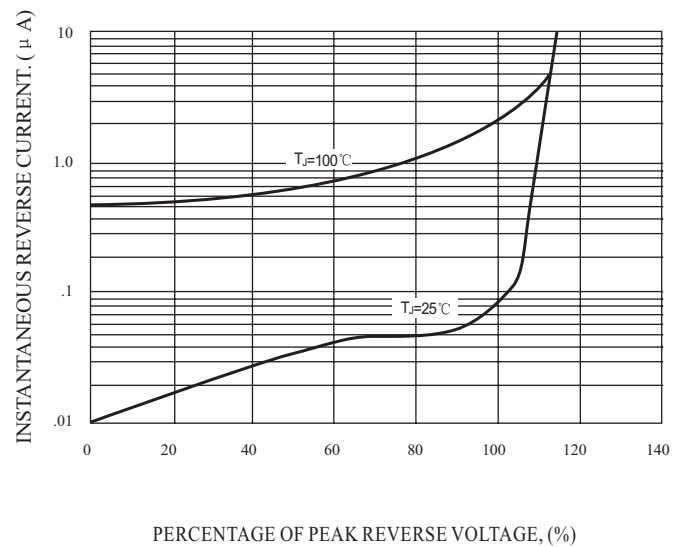
FIG.4-TYPICAL REVERSE CHARACTERISTICS
